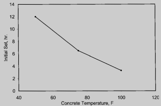
Effect of temperature on concrete setting time (Ref 1)
