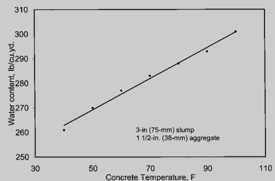
Effect of temperature on water requirement of concrete (Ref 1)
